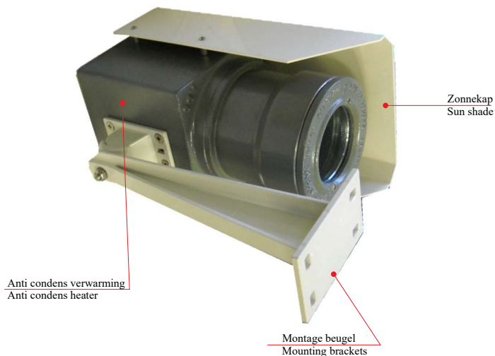
Camerabehuizing Ex d - type INDEX.GUB.CAM Camera box Ex d - type INDEX.GUB.CAM
