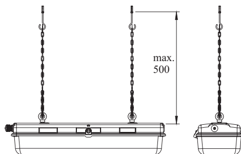
Montage met kettingen Mounting with chains
