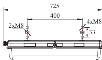
type Z0865 - 2 x 18 Watt
