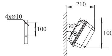
Montage met wandbeugel Mounting with wall bracket
