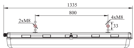
type Z0866 - 2 x 36 Watt
