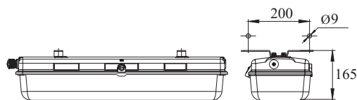
Montage met plafondbeugels Mounting with ceiling brackets
